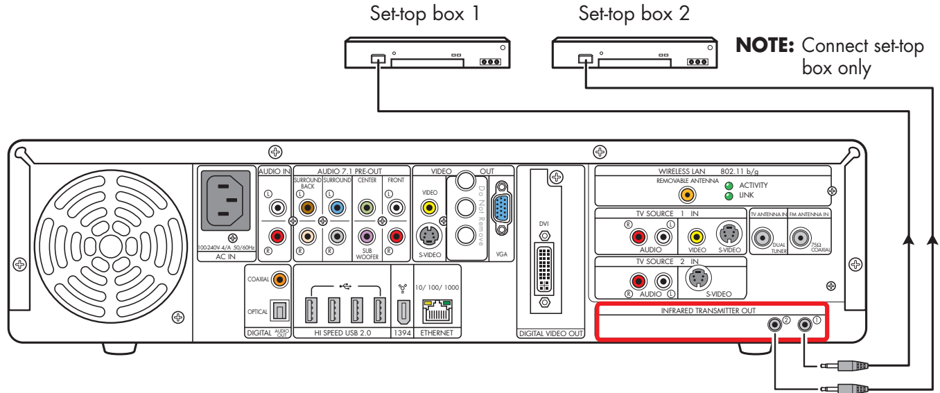
Infrared Transmitter connection (two set-top boxes; select models only)
